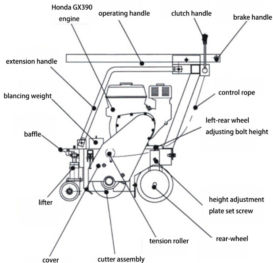
GD-D390 marking removal machine
